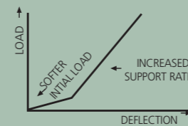
LOAD DEFLECTION ANALYSIS 彈簧負重感應分析
